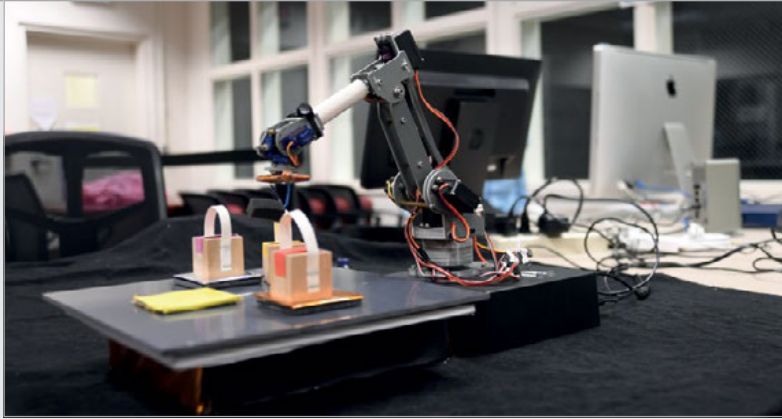
Left The manipulator arm tip can also be equipped with a hook to pick up blocks with loops attached
