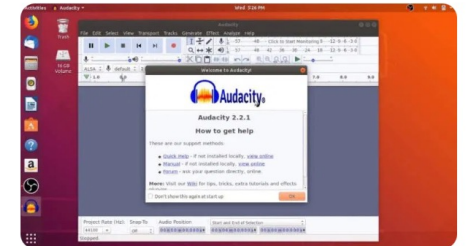
Audacity Linux
