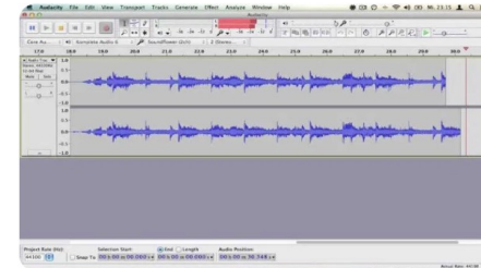
Audacity MacOS
